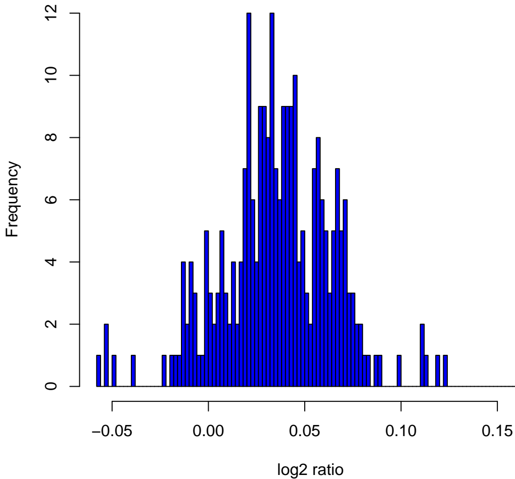
Histogram of log 2 ratios in 270 HapMap samples at clone Chr1tp-10C2
