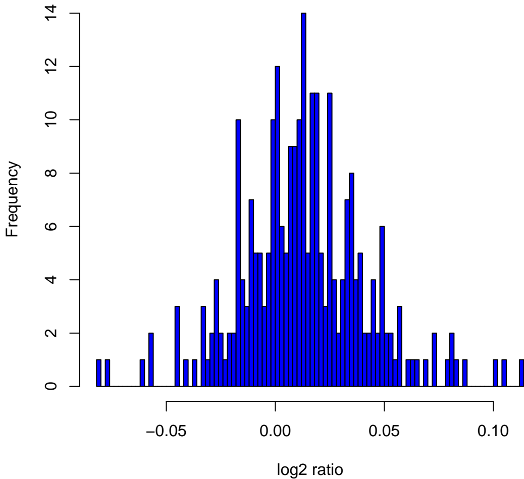
Histogram of log2ratios in 270 HapMap samples at clone Chr1tp-10E10
