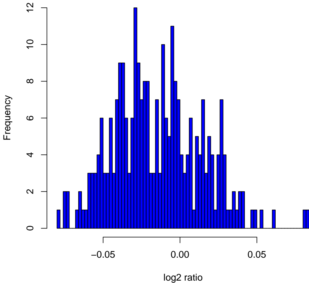
Histogram of log2ratios in 270 HapMap samples at clone Chr1tp-10H12
