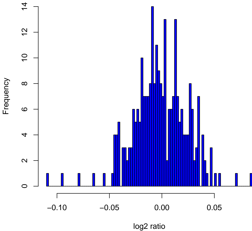
Histogram of log 2 ratios in 270 HapMap samples at clone Chr1tp-11B4
