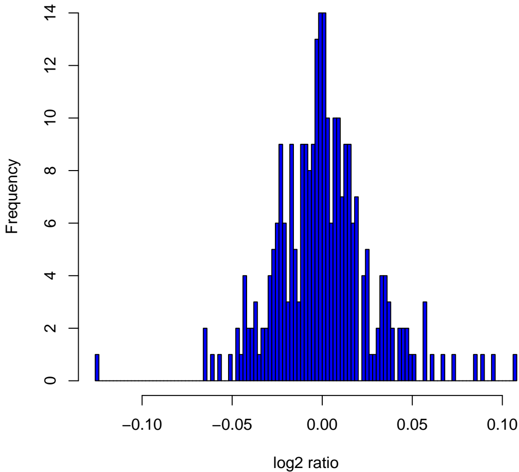
Histogram of log 2 ratios in 270 HapMap samples at clone Chr1tp-11C4
