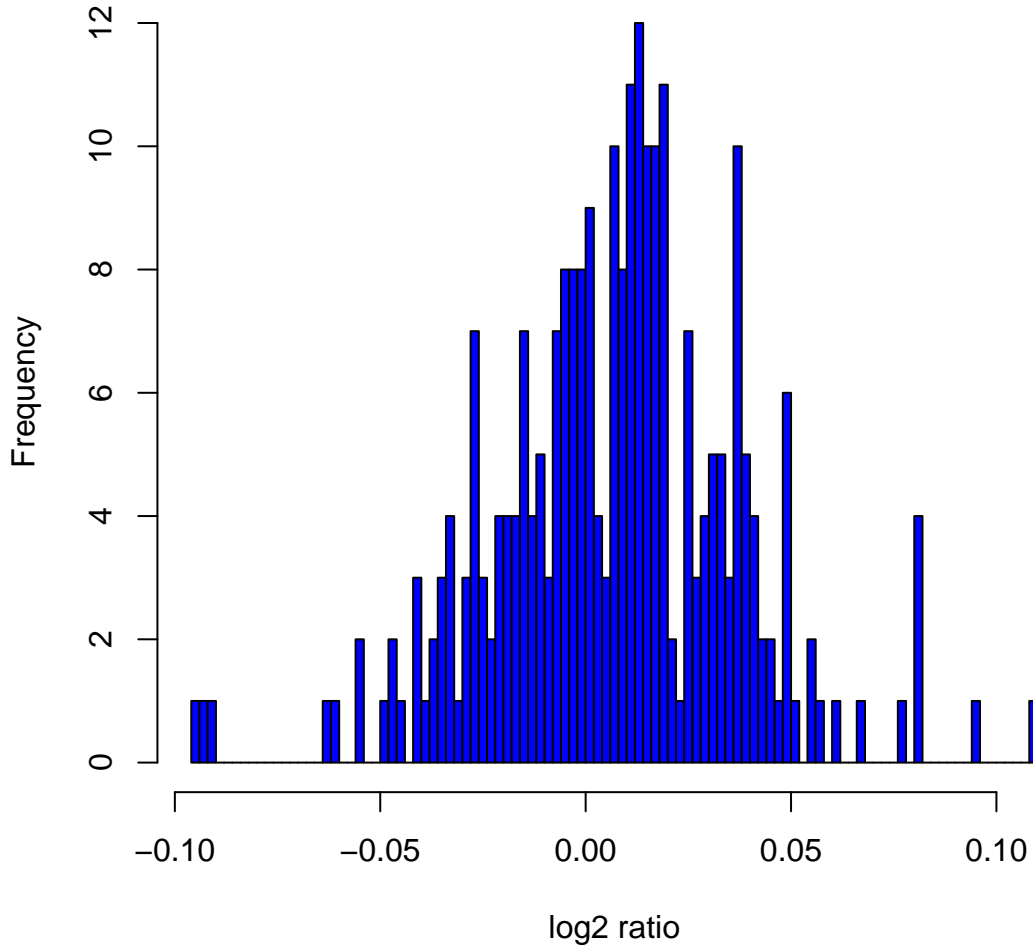
Histogram of log2ratios in 270 HapMap samples at clone Chr1tp-11D11
