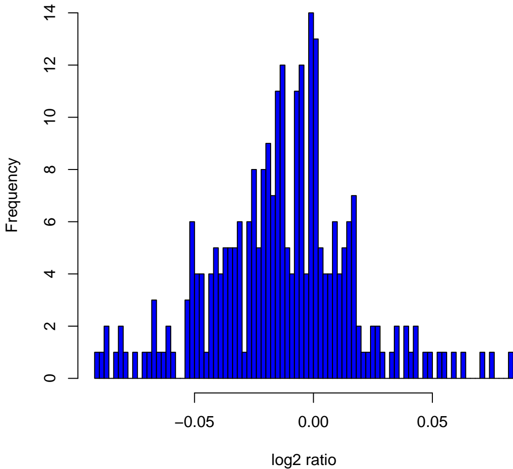
Histogram of log 2 ratios in 270 HapMap samples at clone Chr1tp-11G5
