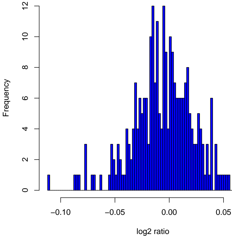
Histogram of \log_2 ratios in 270 HapMap samples at clone Chr1tp-12G5
