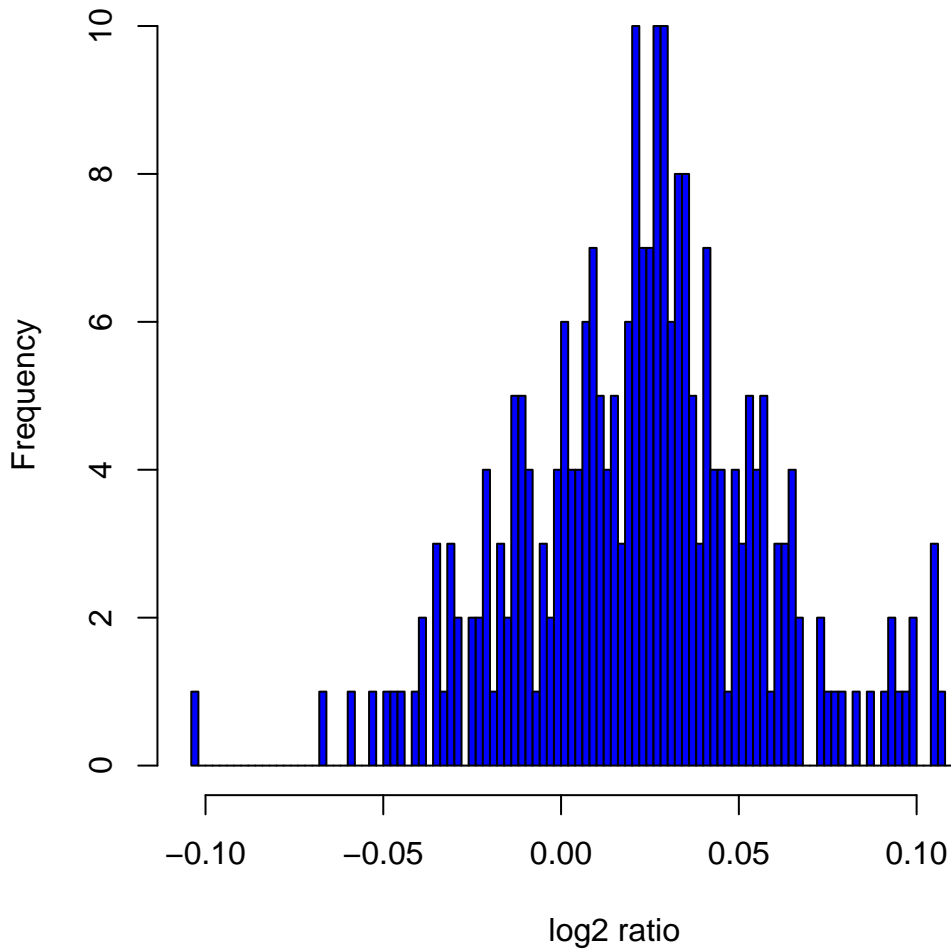
Histogram of log 2 ratios in 270 HapMap samples at clone Chr1tp-12H1
