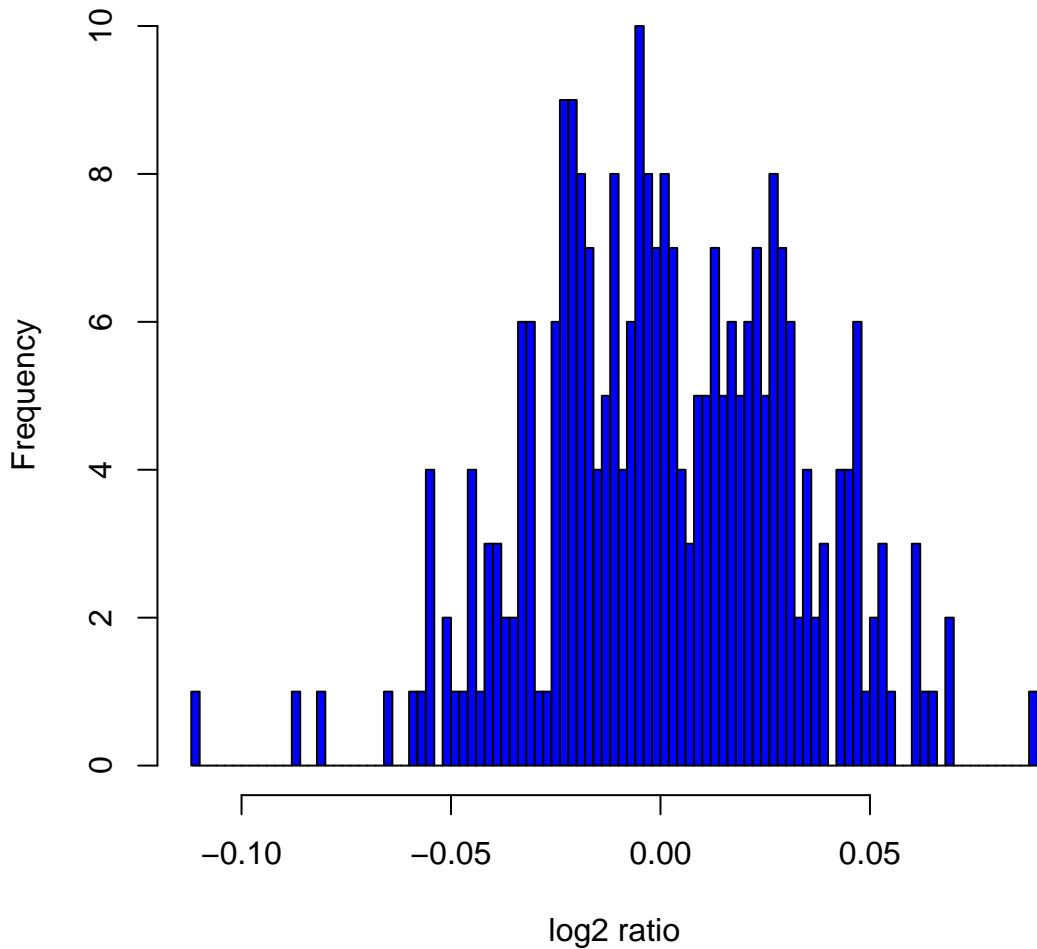
Histogram of \log_2 ratios in 270 HapMap samples at clone Chr1tp-13G1
