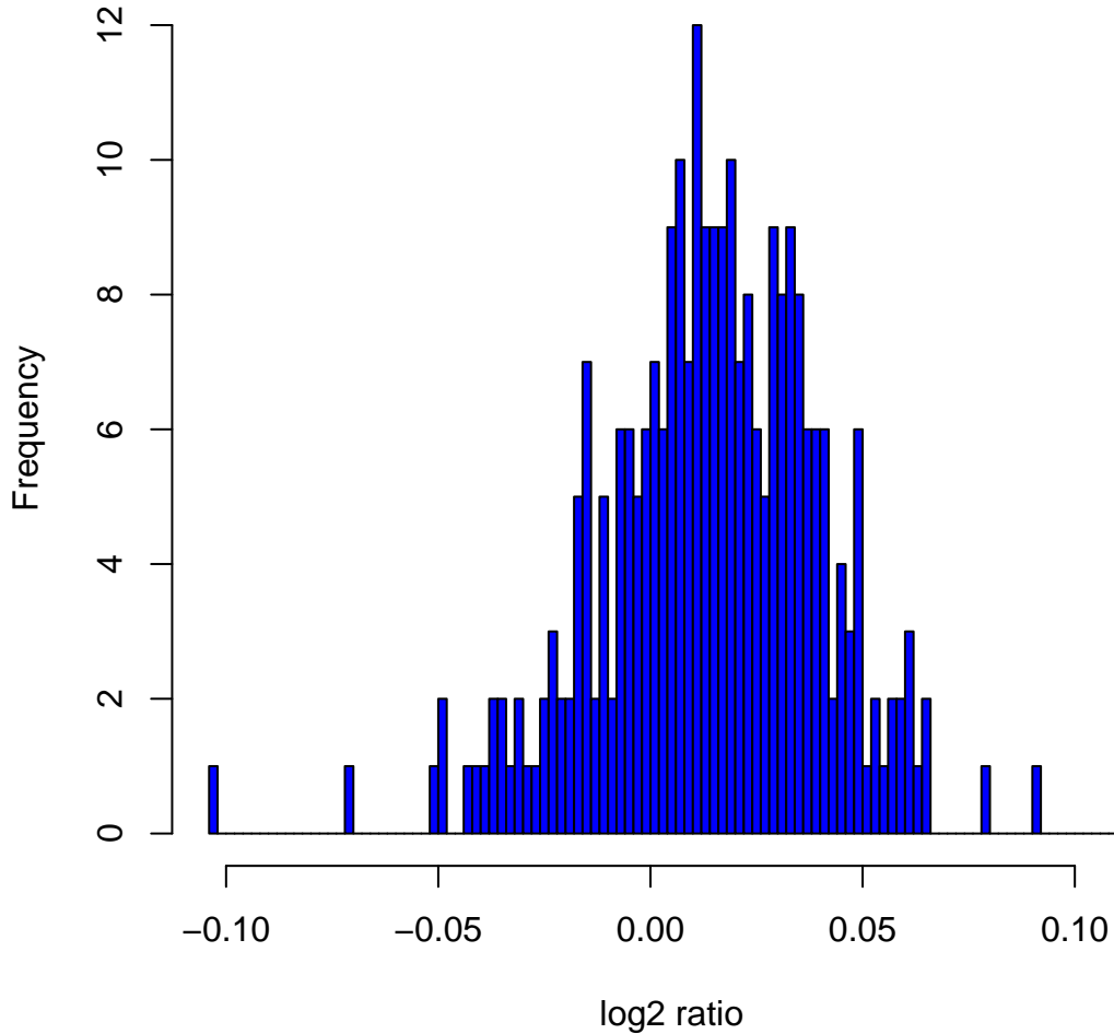
Histogram of log 2 ratios in 270 HapMap samples at clone Chr1tp-13G2
