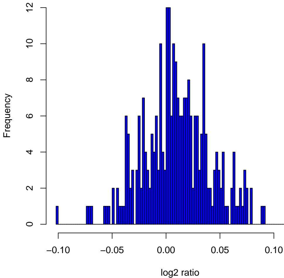
Histogram of log 2 ratios in 270 HapMap samples at clone Chr1tp-14A3
