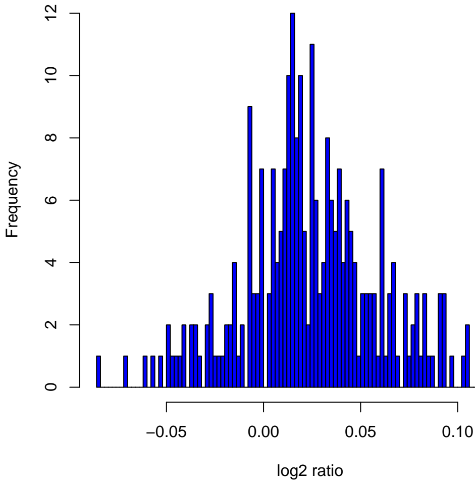
Histogram of log 2 ratios in 270 HapMap samples at clone Chr1tp-14B7
