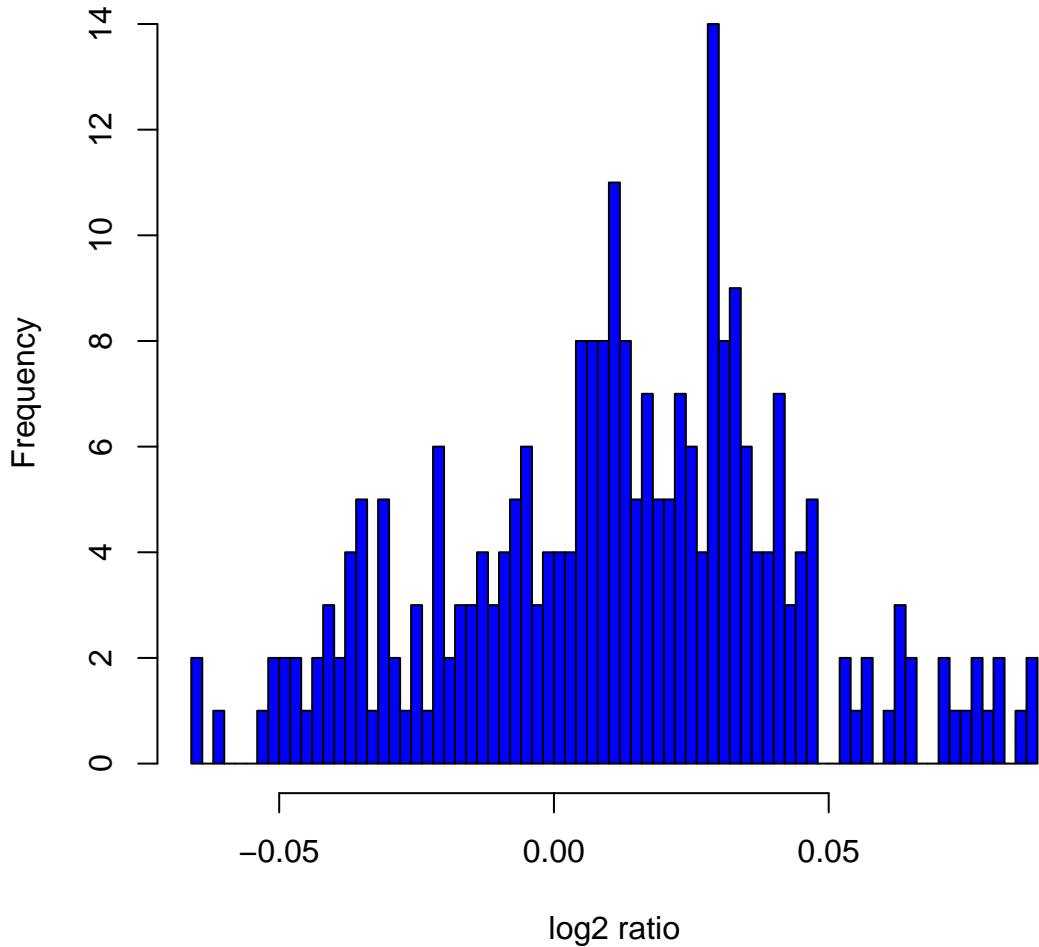
Histogram of log 2 ratios in 270 HapMap samples at clone Chr1tp-14D6
