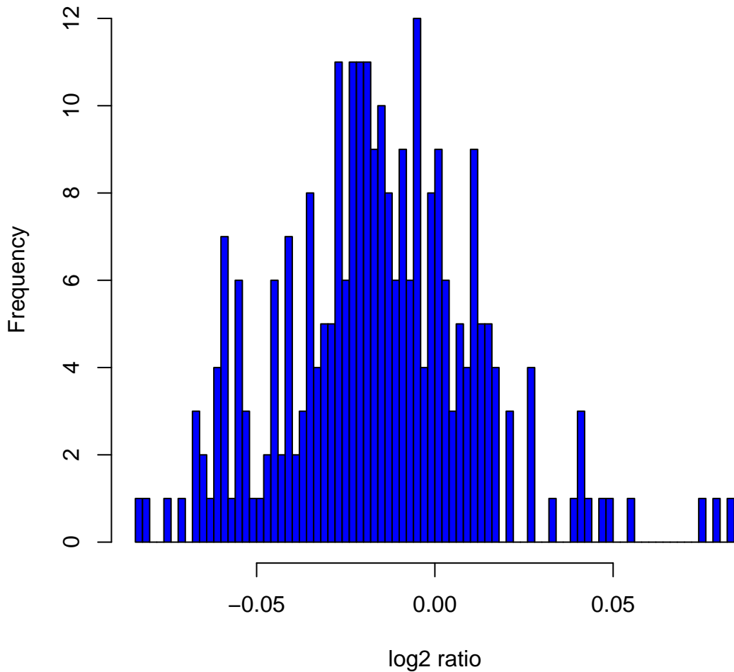
Histogram of log2ratios in 270 HapMap samples at clone Chr1tp-14E10
