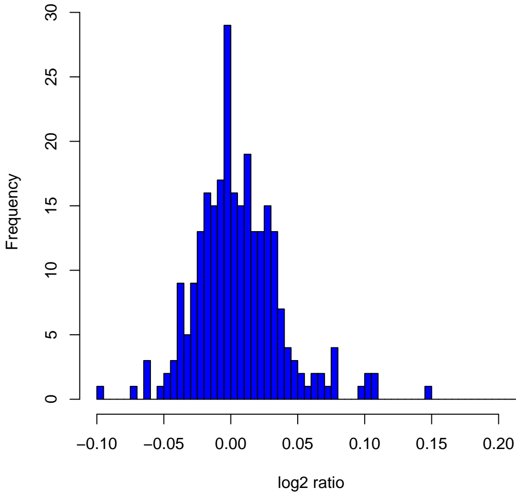
Histogram of log2ratios in 270 HapMap samples at clone Chr1tp-14F11
