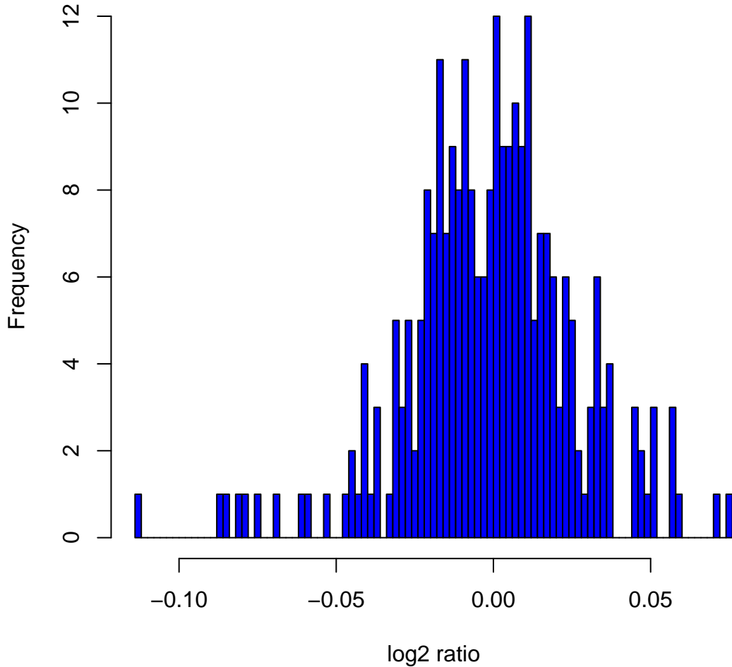
Histogram of log 2 ratios in 270 HapMap samples at clone Chr1tp-14G8
