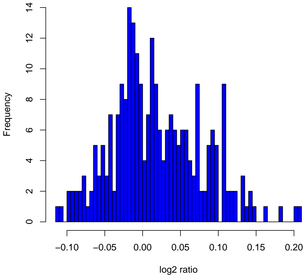
Histogram of log 2 ratios in 270 HapMap samples at clone Chr1tp-14H2
