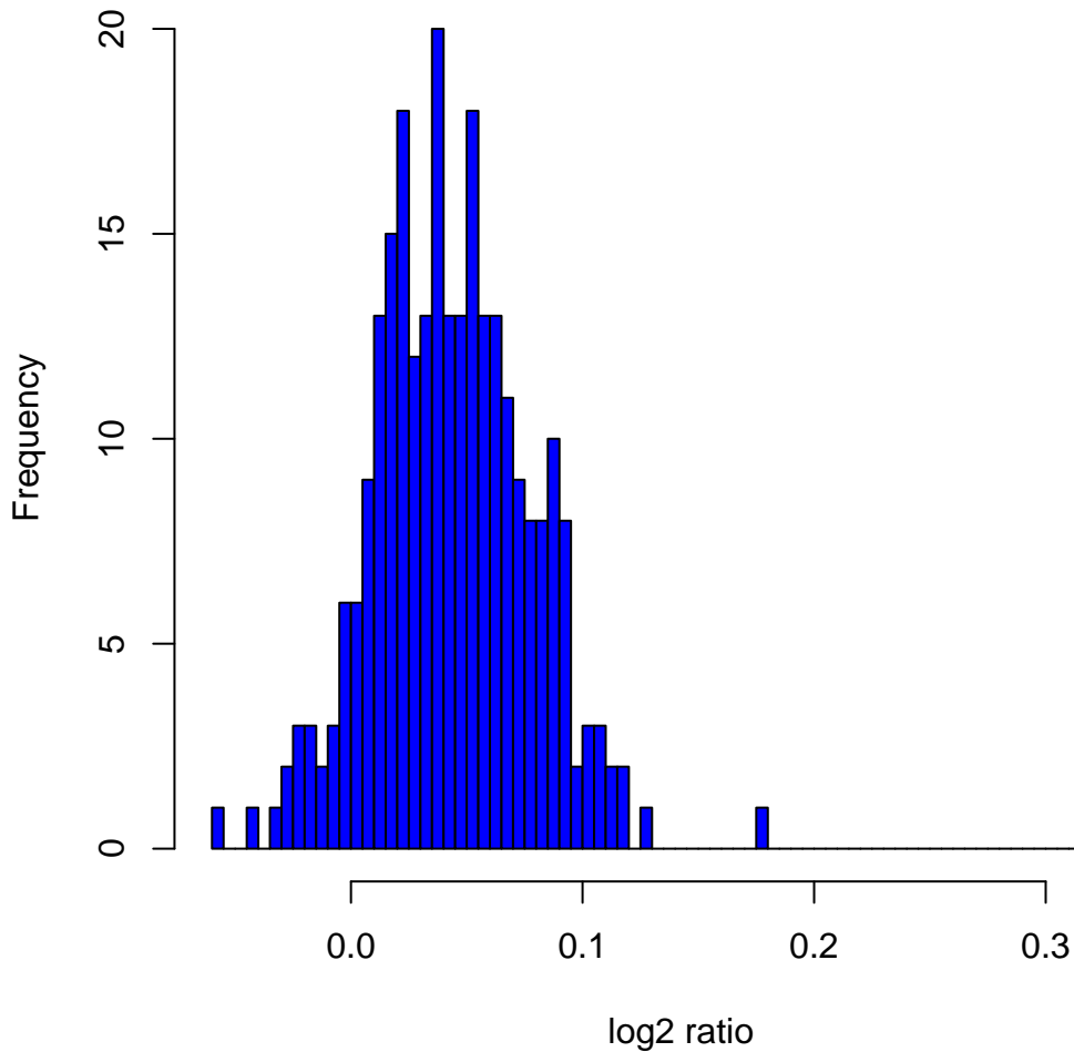
Histogram of log 2 ratios in 270 HapMap samples at clone Chr1tp-15A3
