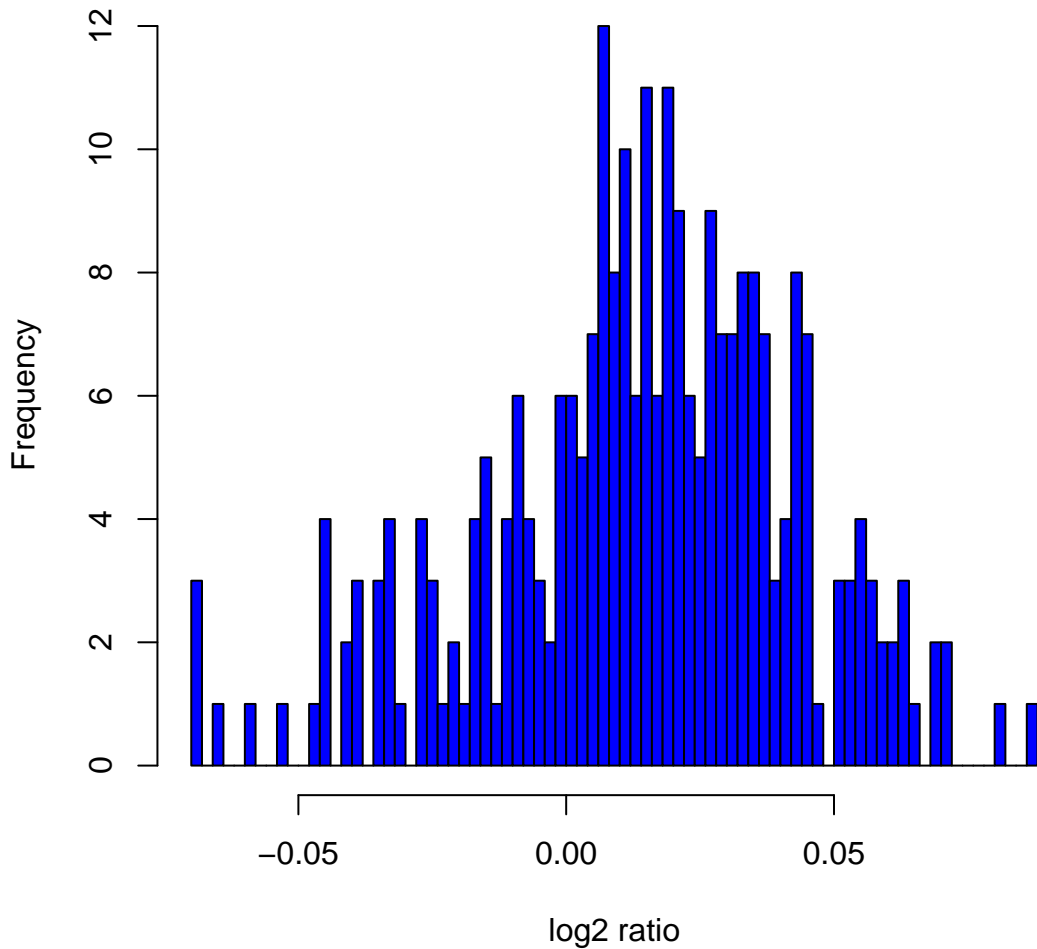
Histogram of log2ratios in 270 HapMap samples at clone Chr1tp-16A12
