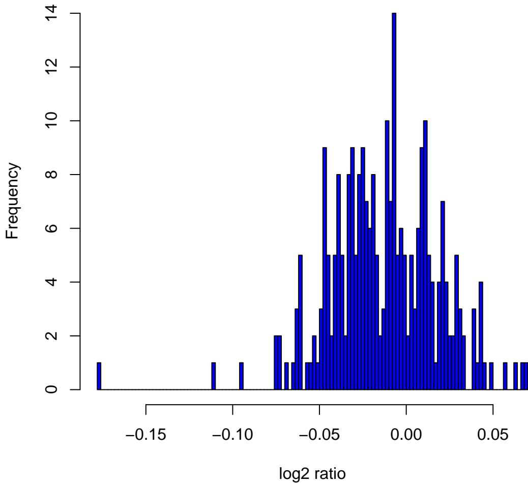
Histogram of log2ratios in 270 HapMap samples at clone Chr1tp-18C12
