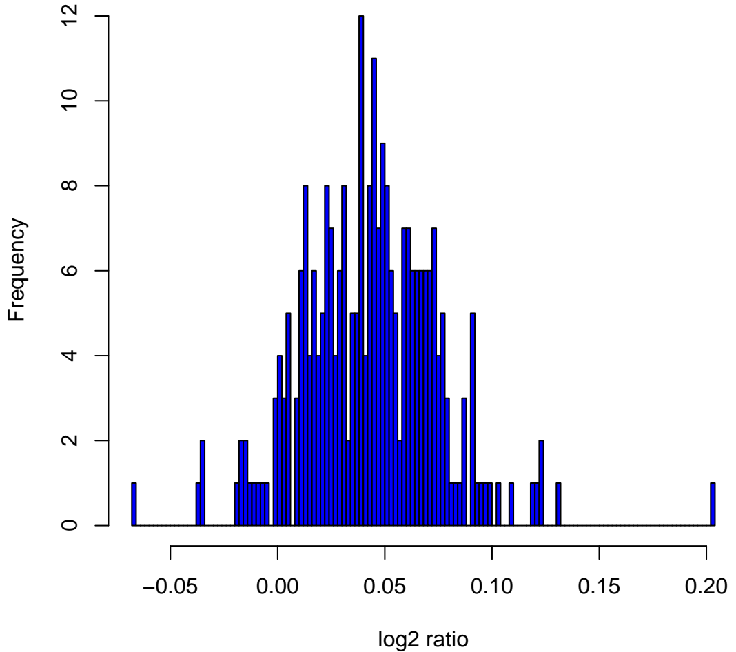
Histogram of log2ratios in 270 HapMap samples at clone Chr1tp-18E11
