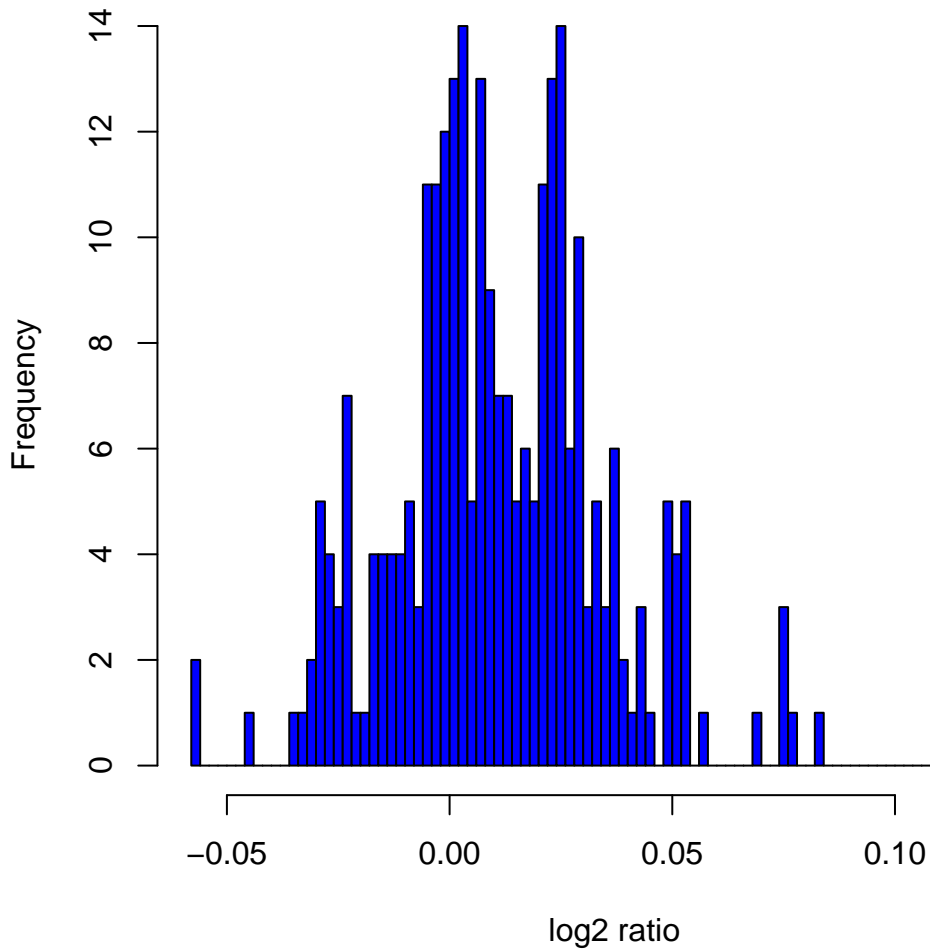
Histogram of log2ratios in 270 HapMap samples at clone Chr1tp-18F11
