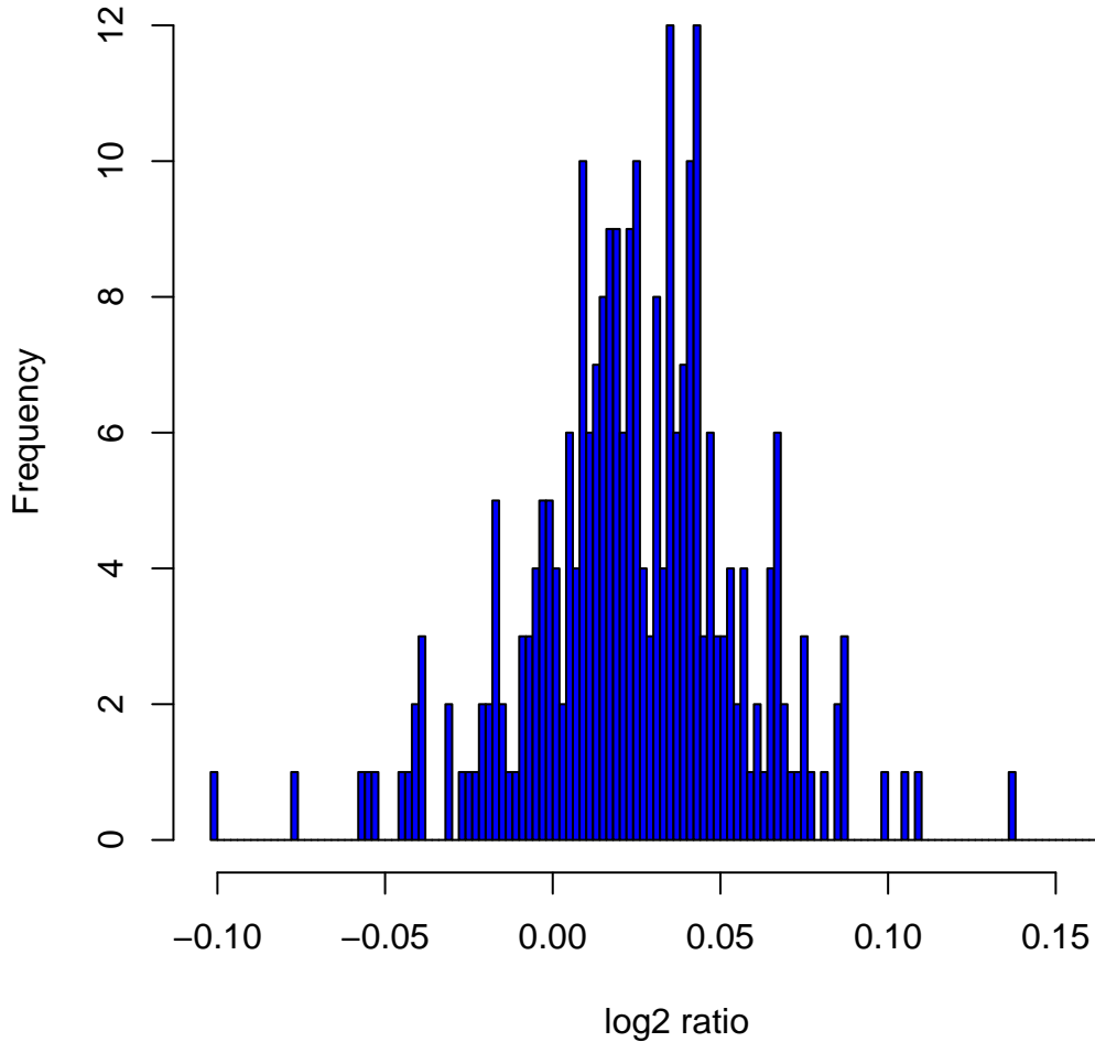
Histogram of log 2 ratios in 270 HapMap samples at clone Chr1tp-19B6
