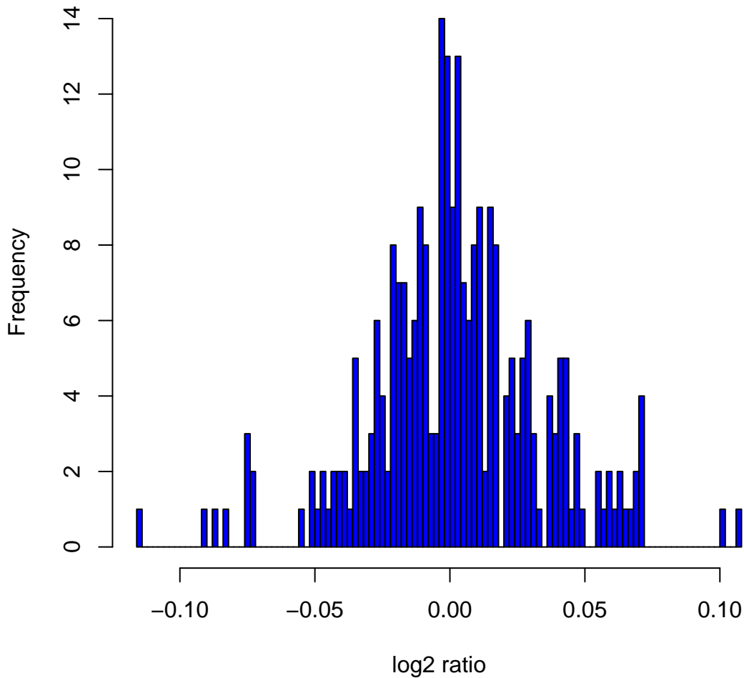
Histogram of log 2 ratios in 270 HapMap samples at clone Chr1tp-19C3
