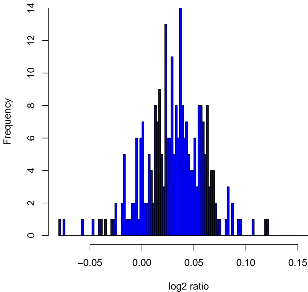
Histogram of log 2 ratios in 270 HapMap samples at clone Chr1tp-19C5
