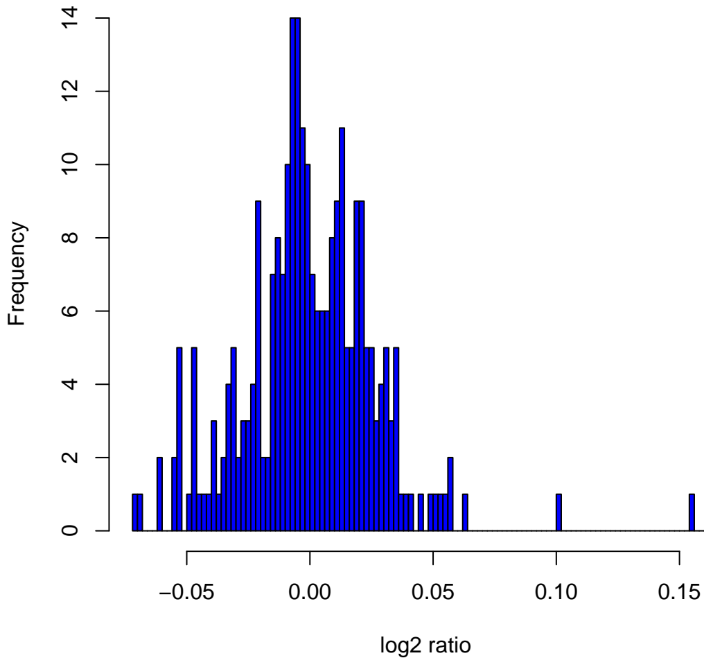
Histogram of \log_2 ratios in 270 HapMap samples at clone Chr1tp-19D2
