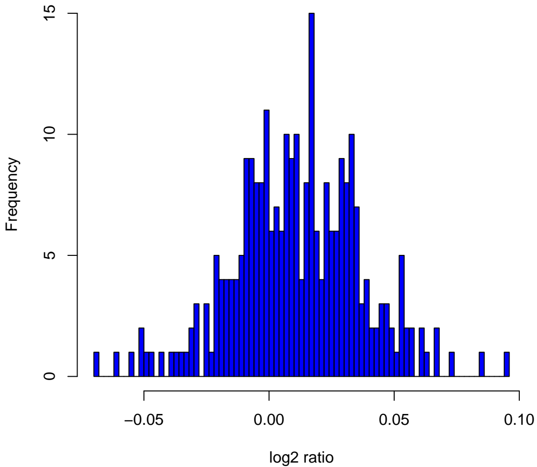
Histogram of log 2 ratios in 270 HapMap samples at clone Chr1tp-19E8
