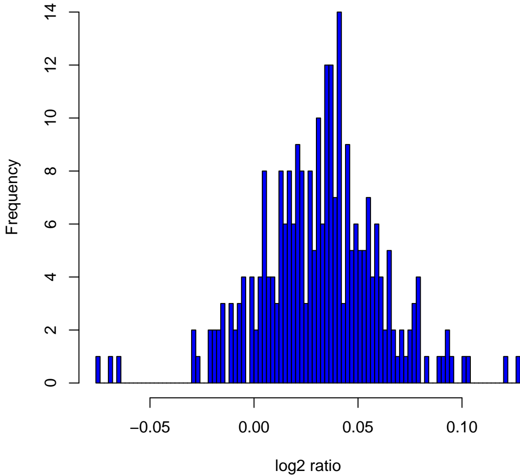
Histogram of log 2 ratios in 270 HapMap samples at clone Chr1tp-19G3
