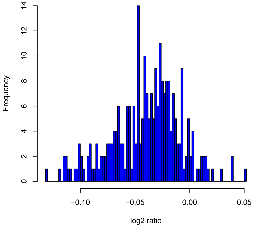
Histogram of log 2 ratios in 270 HapMap samples at clone Chr1tp-19G8
