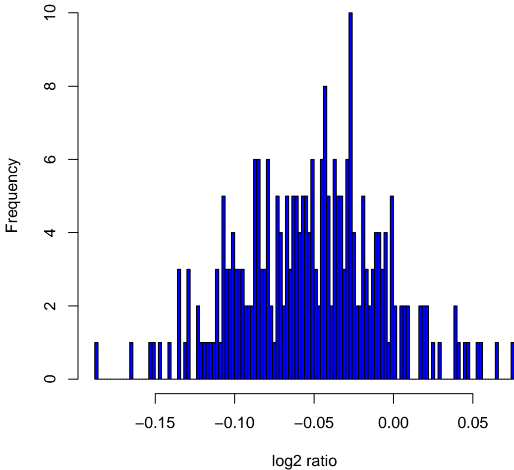
Histogram of \log_2 ratios in 270 HapMap samples at clone Chr1tp-1B5
