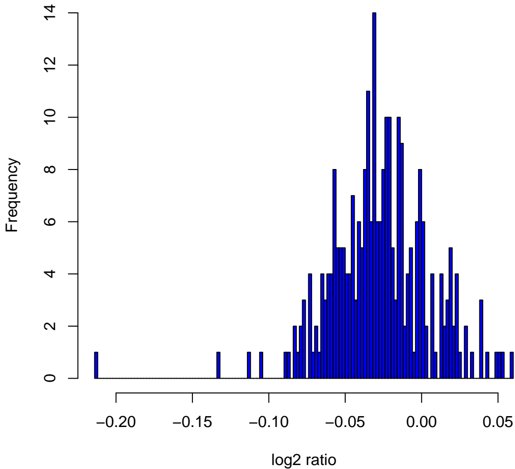
Histogram of log 2 ratios in 270 HapMap samples at clone Chr1tp-1C9
