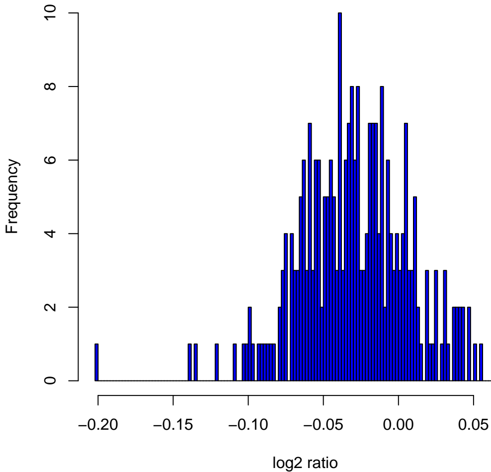
Histogram of log 2 ratios in 270 HapMap samples at clone Chr1tp-1D2
