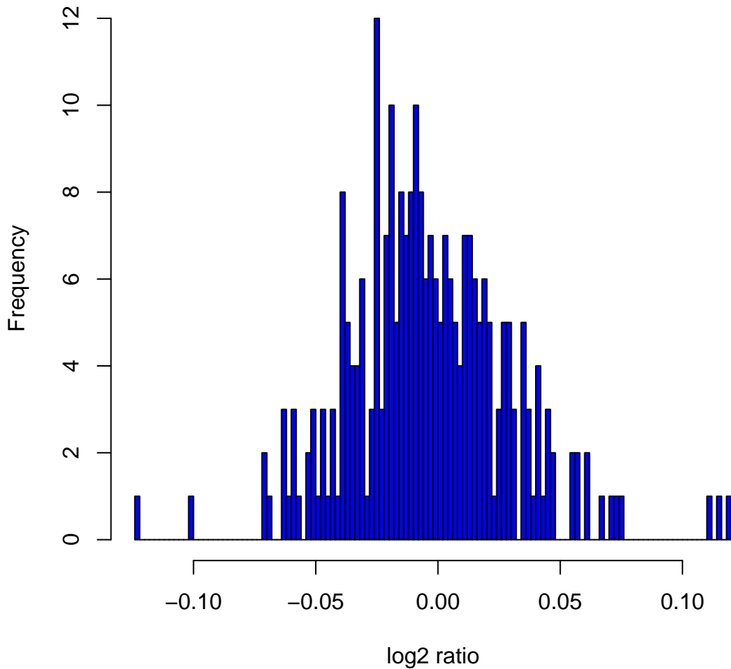
Histogram of log 2 ratios in 270 HapMap samples at clone Chr1tp-1D9
