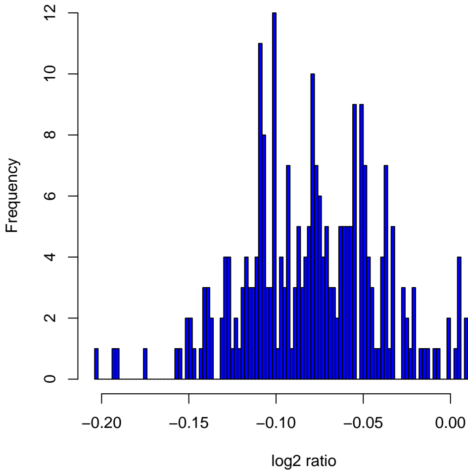
Histogram of \log_2 ratios in 270 HapMap samples at clone Chr1tp-1E7
