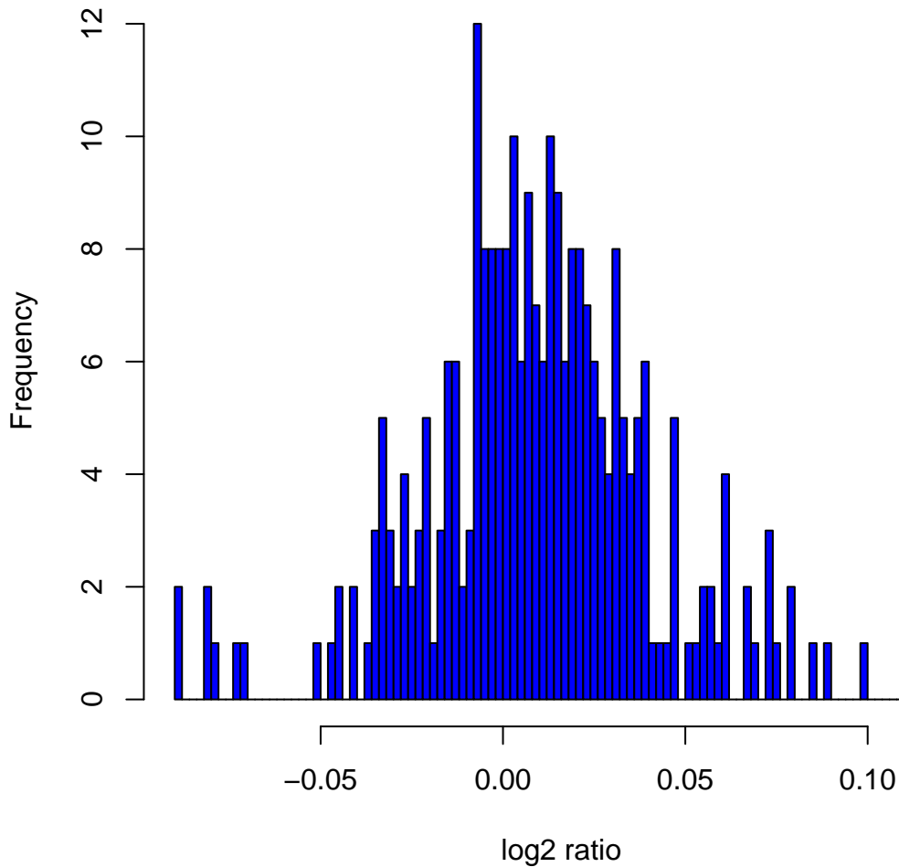
Histogram of log2ratios in 270 HapMap samples at clone Chr1tp-1F9
