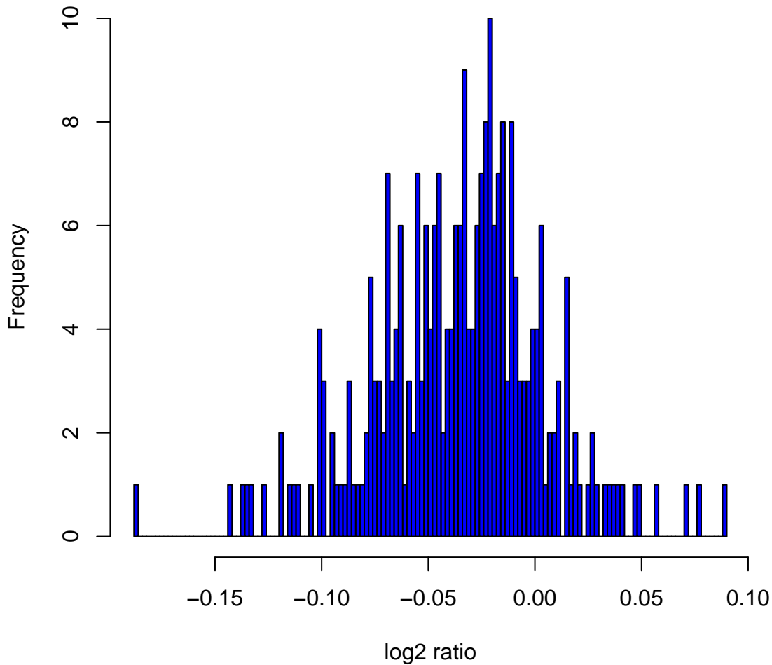
Histogram of \log_2 ratios in 270 HapMap samples at clone Chr1tp-1G11
