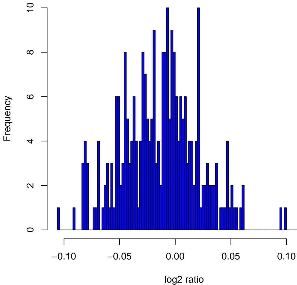
Histogram of log 2 ratios in 270 HapMap samples at clone Chr1tp-1H3
