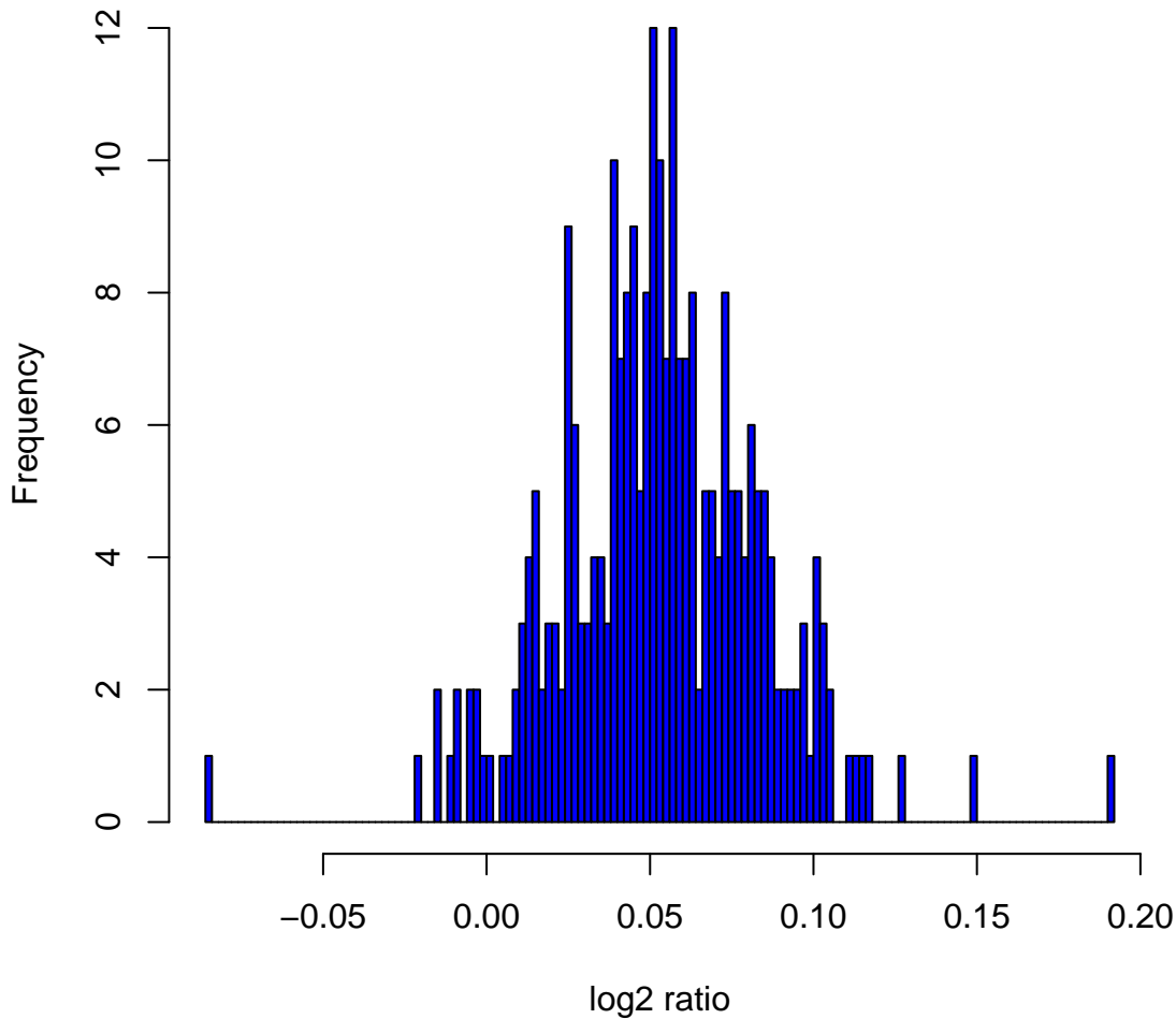
Histogram of log2ratios in 270 HapMap samples at clone Chr1tp-20A10
