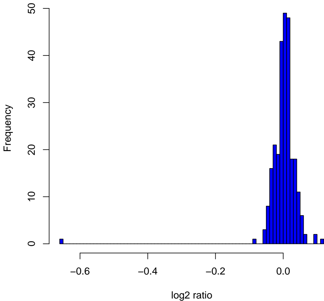
Histogram of log2ratios in 270 HapMap samples at clone Chr1tp-20E8
