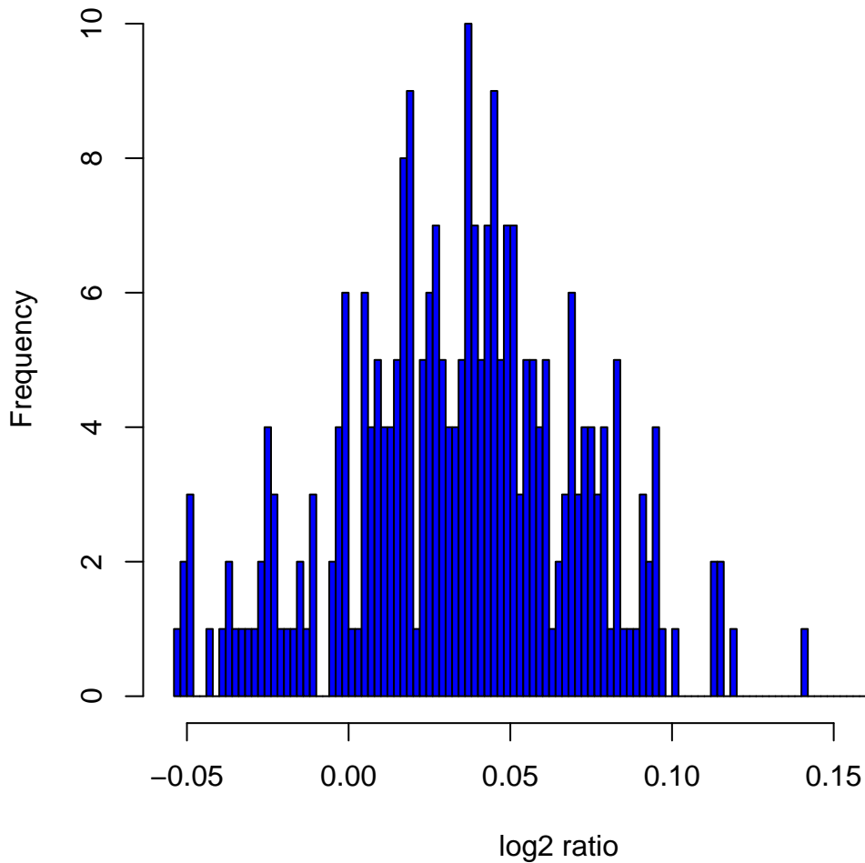
Histogram of log 2 ratios in 270 HapMap samples at clone Chr1tp-20G7
