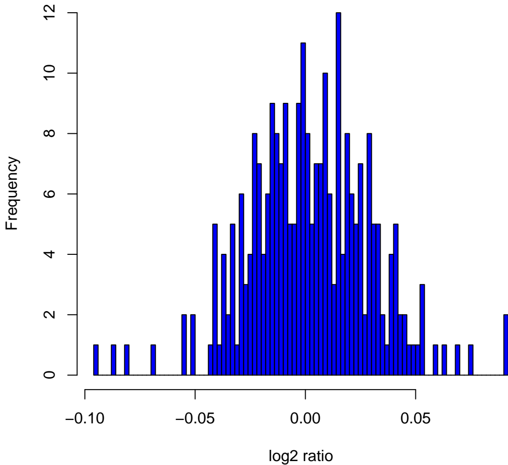
Histogram of log 2 ratios in 270 HapMap samples at clone Chr1tp-21D4
