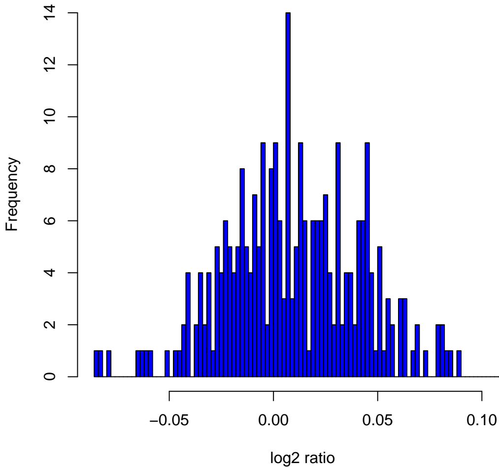
Histogram of log 2 ratios in 270 HapMap samples at clone Chr1tp-21F7
