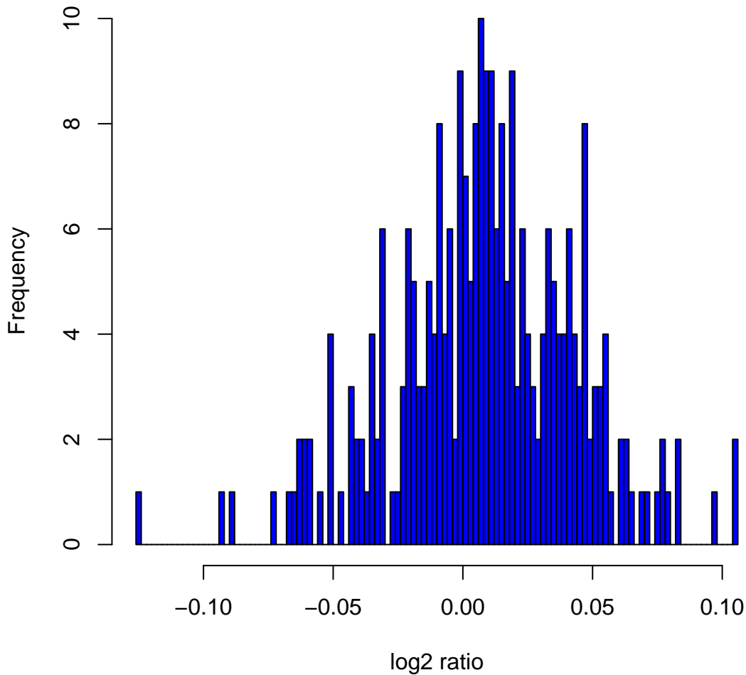
Histogram of log 2 ratios in 270 HapMap samples at clone Chr1tp-22A4
