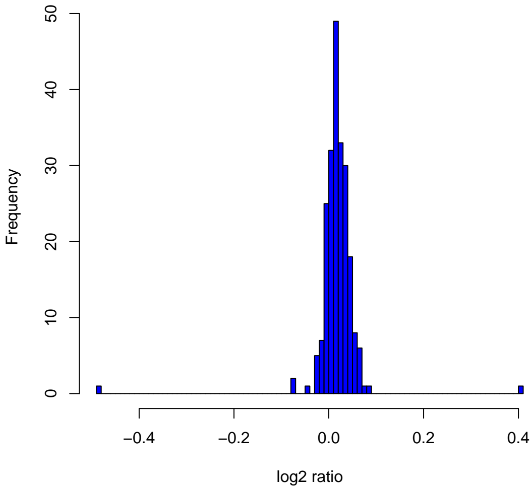
Histogram of log2ratios in 270 HapMap samples at clone Chr1tp-23C6
