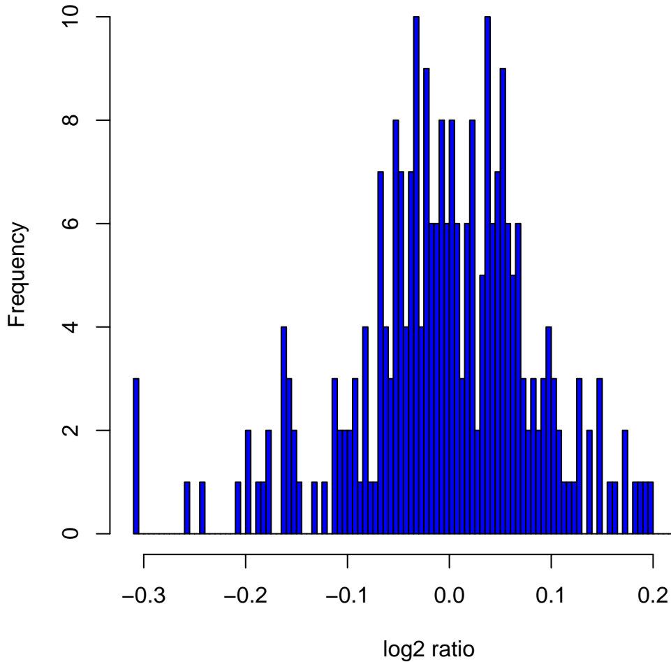
Histogram of log 2 ratios in 270 HapMap samples at clone Chr1tp-23C7
