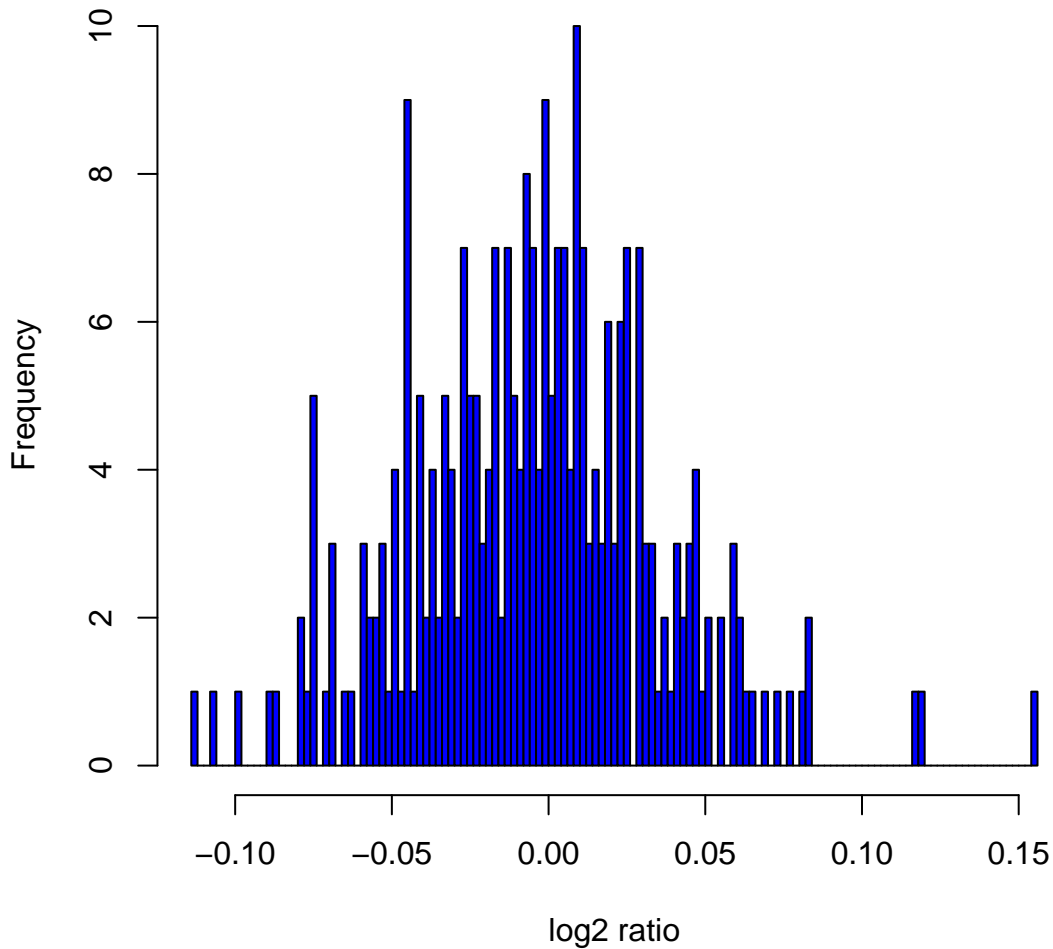
Histogram of log 2 ratios in 270 HapMap samples at clone Chr1tp-23G3
