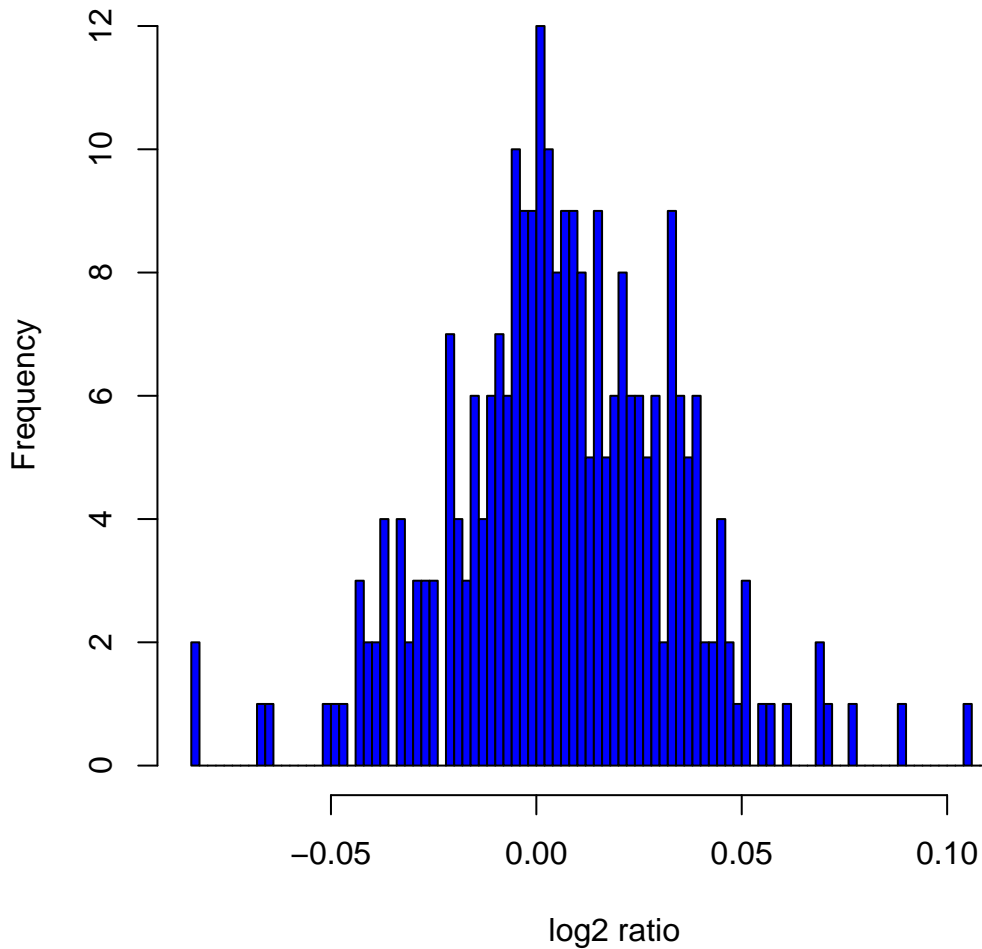
Histogram of log2ratios in 270 HapMap samples at clone Chr1tp-25B12
