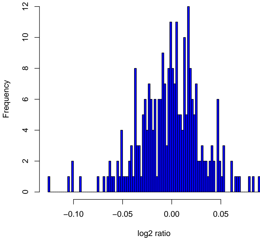
Histogram of log 2 ratios in 270 HapMap samples at clone Chr1tp-25D8
