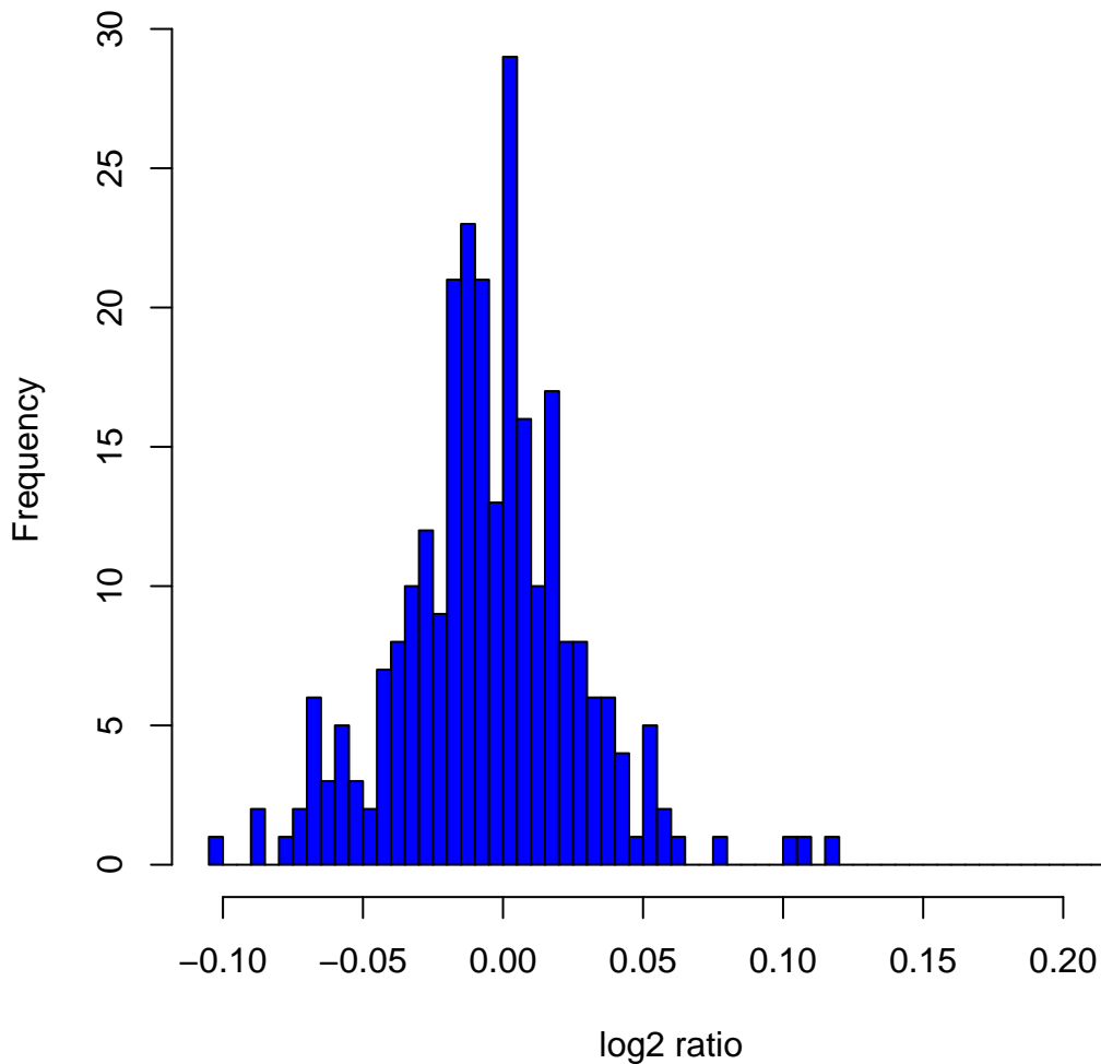
Histogram of \log_2 ratios in 270 HapMap samples at clone Chr1tp-25E1
